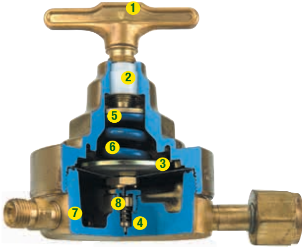
Typical Single Stage Design SH 450 Series Shown 2.5" (63.5 mm) Brass Gauges External Relief Valve System
