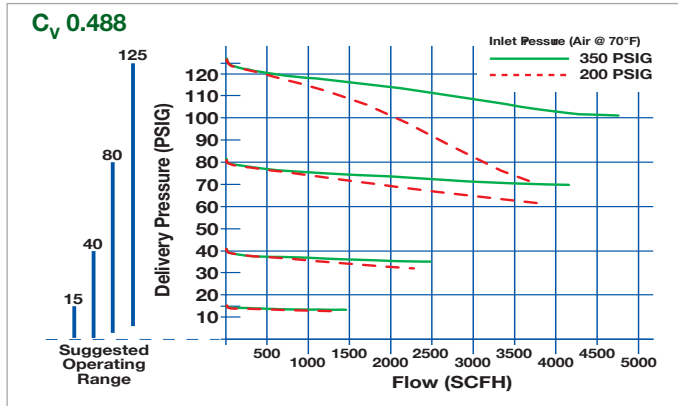
ESL4 FLOW DATA - EDGE Series-Line
