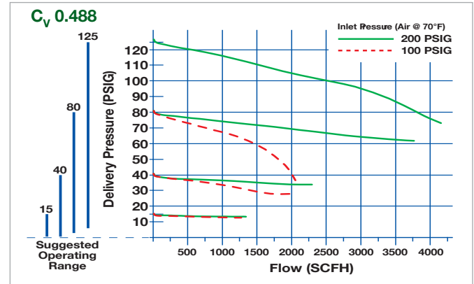
EST4 FLOW DATA - EDGE Series-Station
